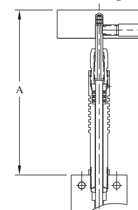
Finned Bonnet
